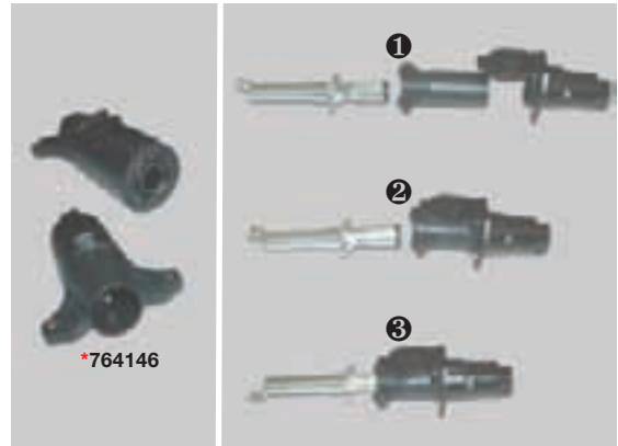
7-Pole to 6-Pole RV Connector Adapter
