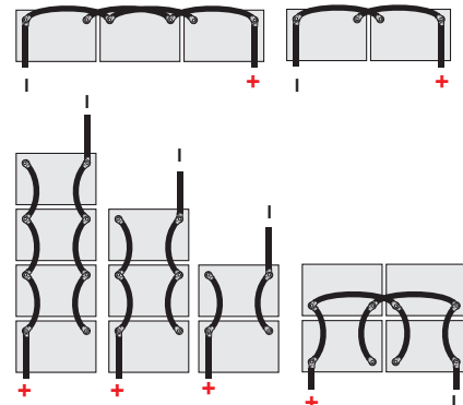
Typical Group 31 layouts
